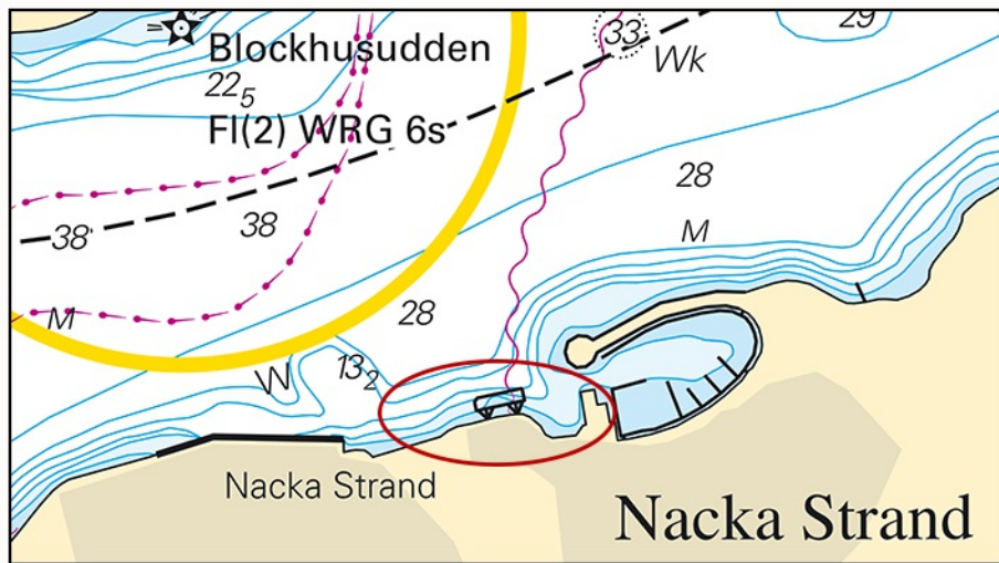
New pontoon jetty at Nacka strand in Stockholm
